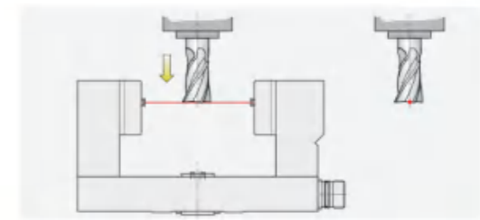
Detection of tool breakage
